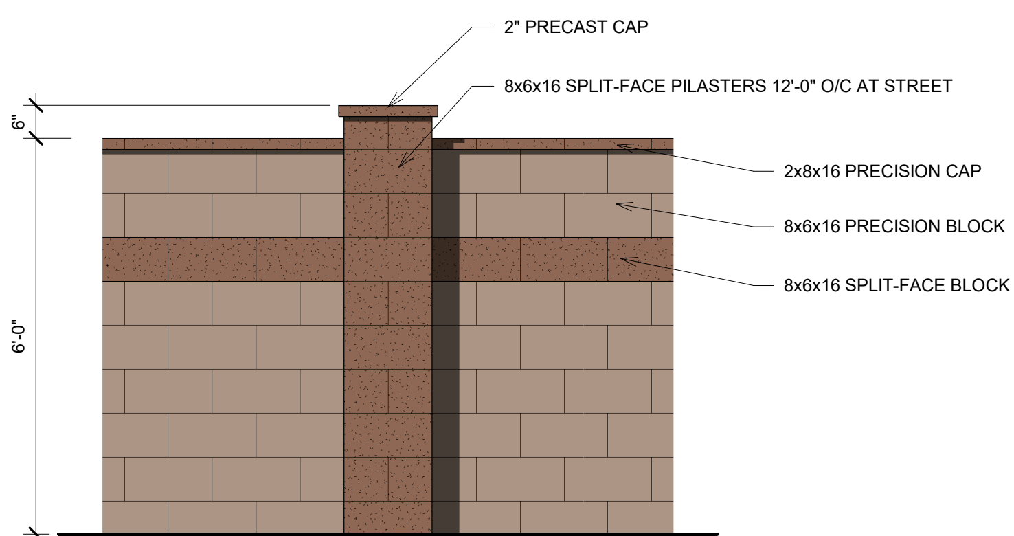
Property Wall 1/2" = 1'-0"
