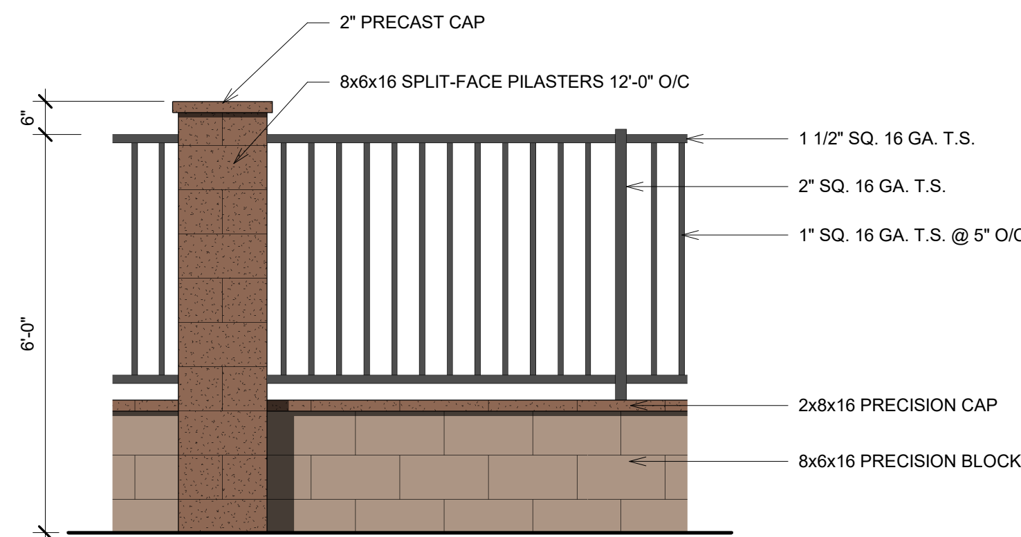
Screen Wall 1/2" = 1'-0"
