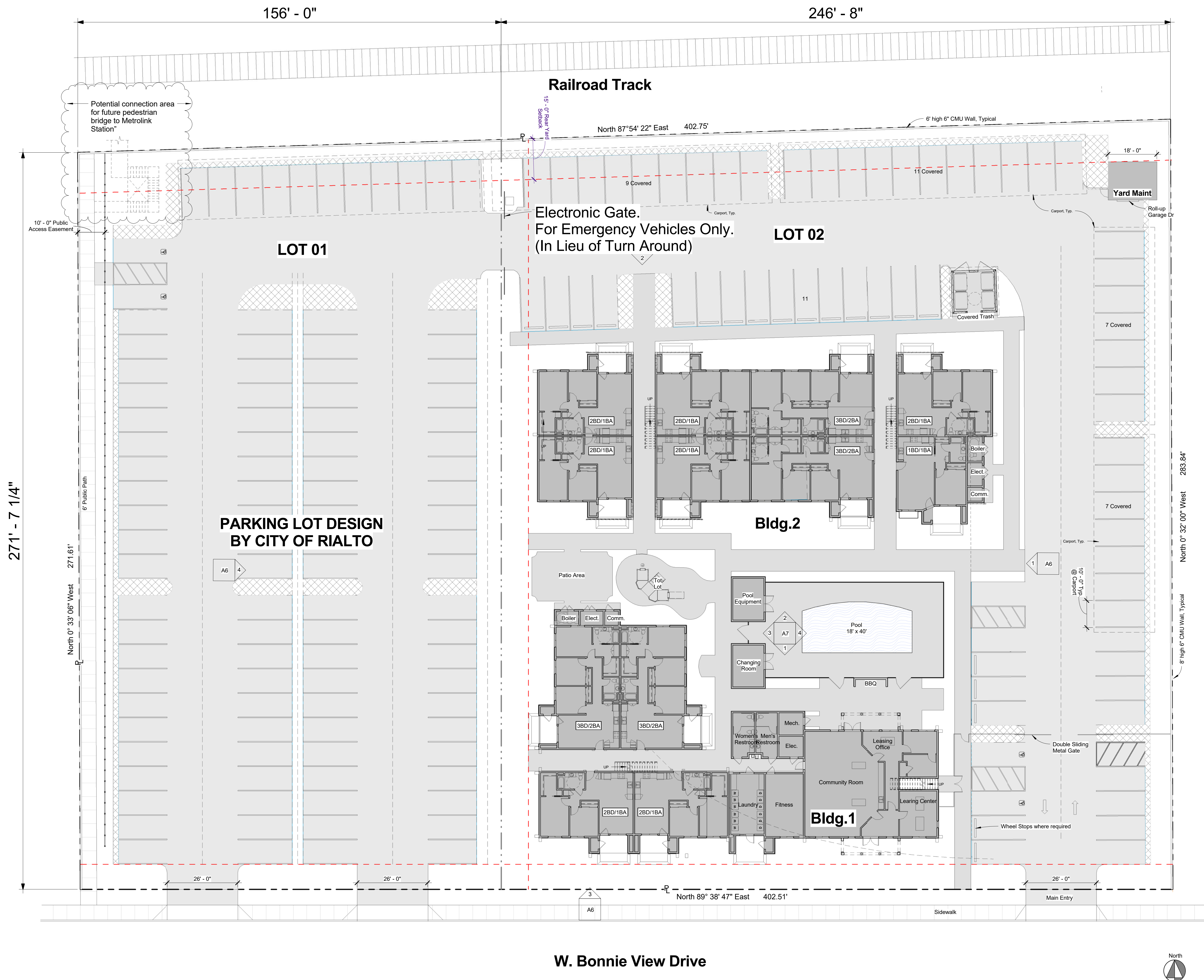
① Site Plan 1/16" = 1'-0"
