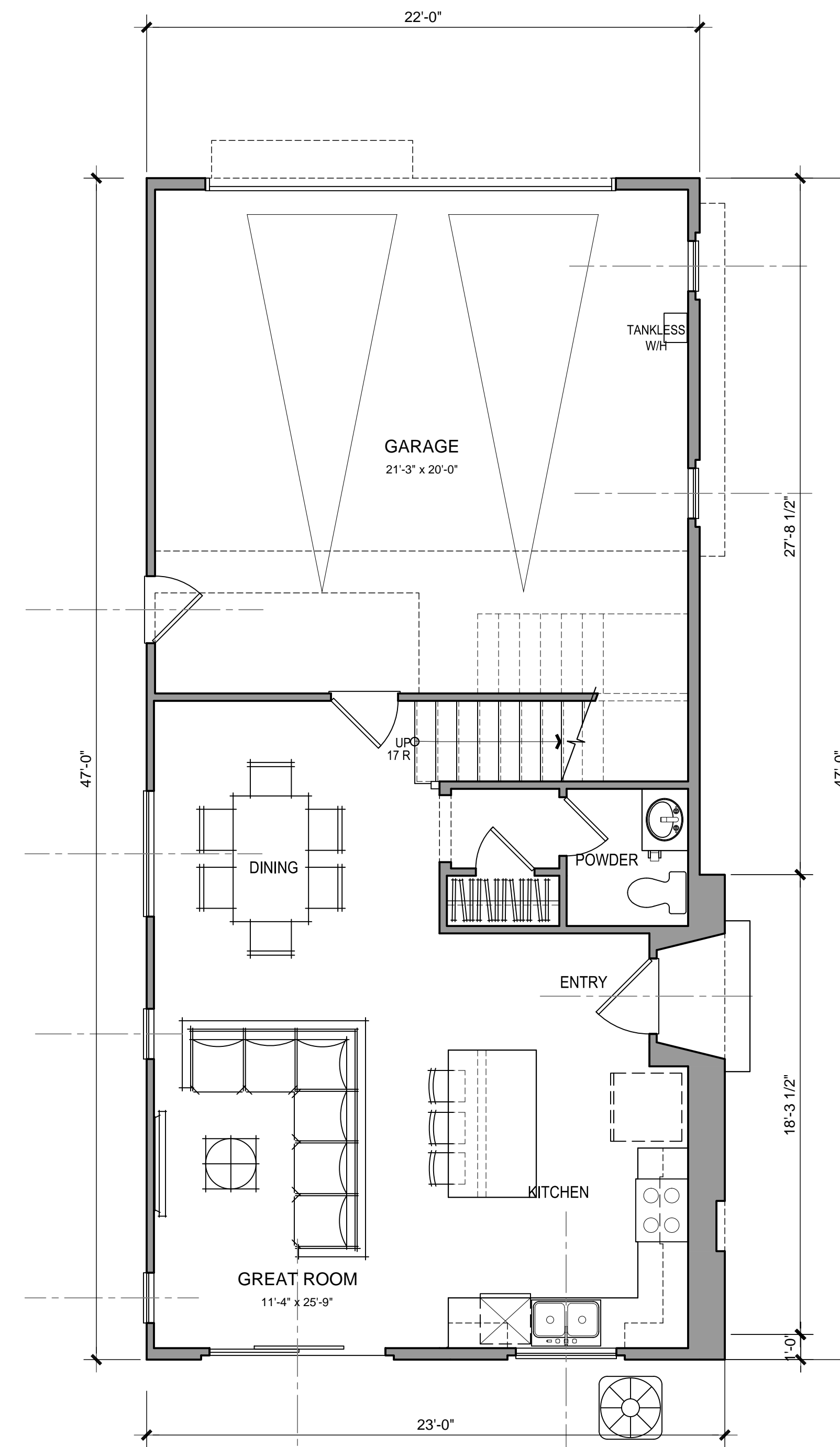
1ST FLOOR PLAN 3BX
