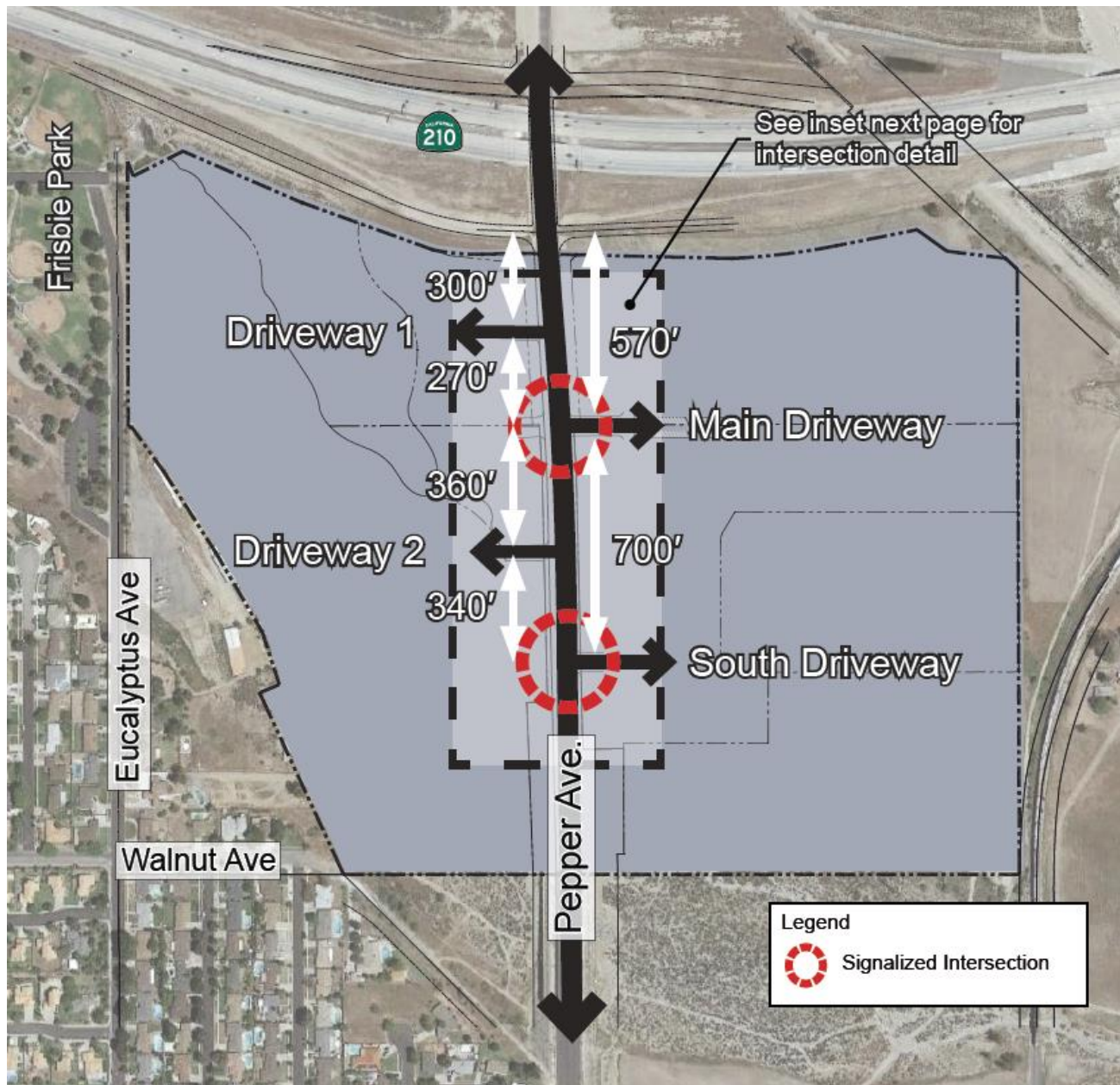
Figure 3-3a Circulation Plan
