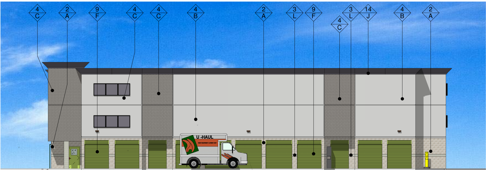
WEST ELEVATION
