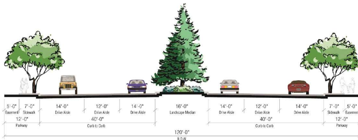
Exhibit 4.12 - Street Section
